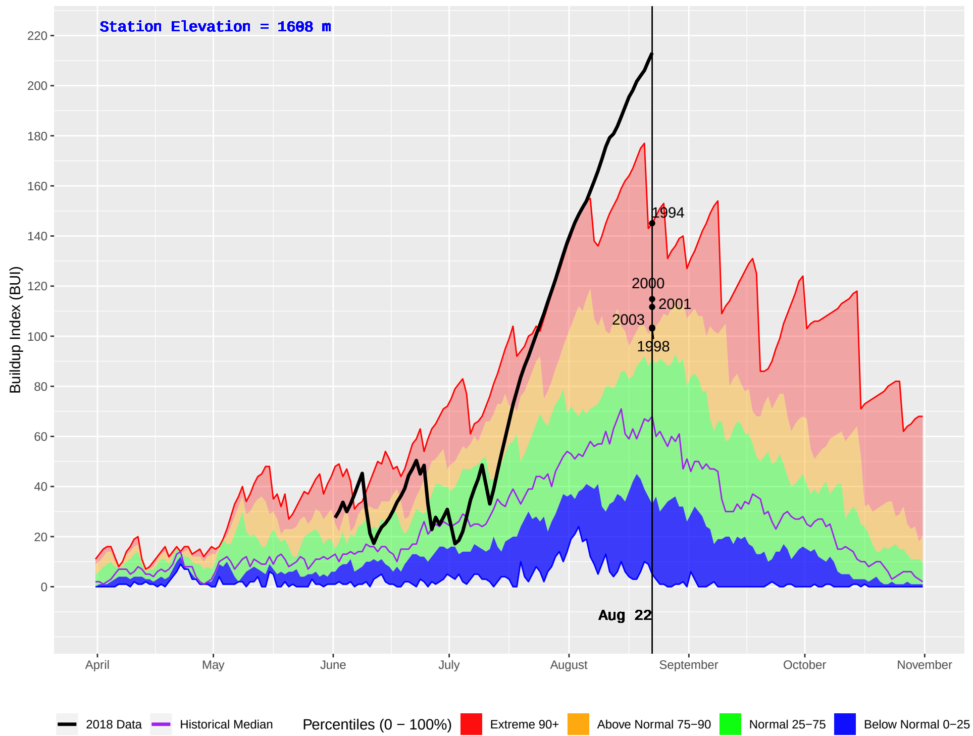
DEWAR CREEK (421) : Historical (1986–2016) and Current (2018) Daily Buildup Index (BUI)
