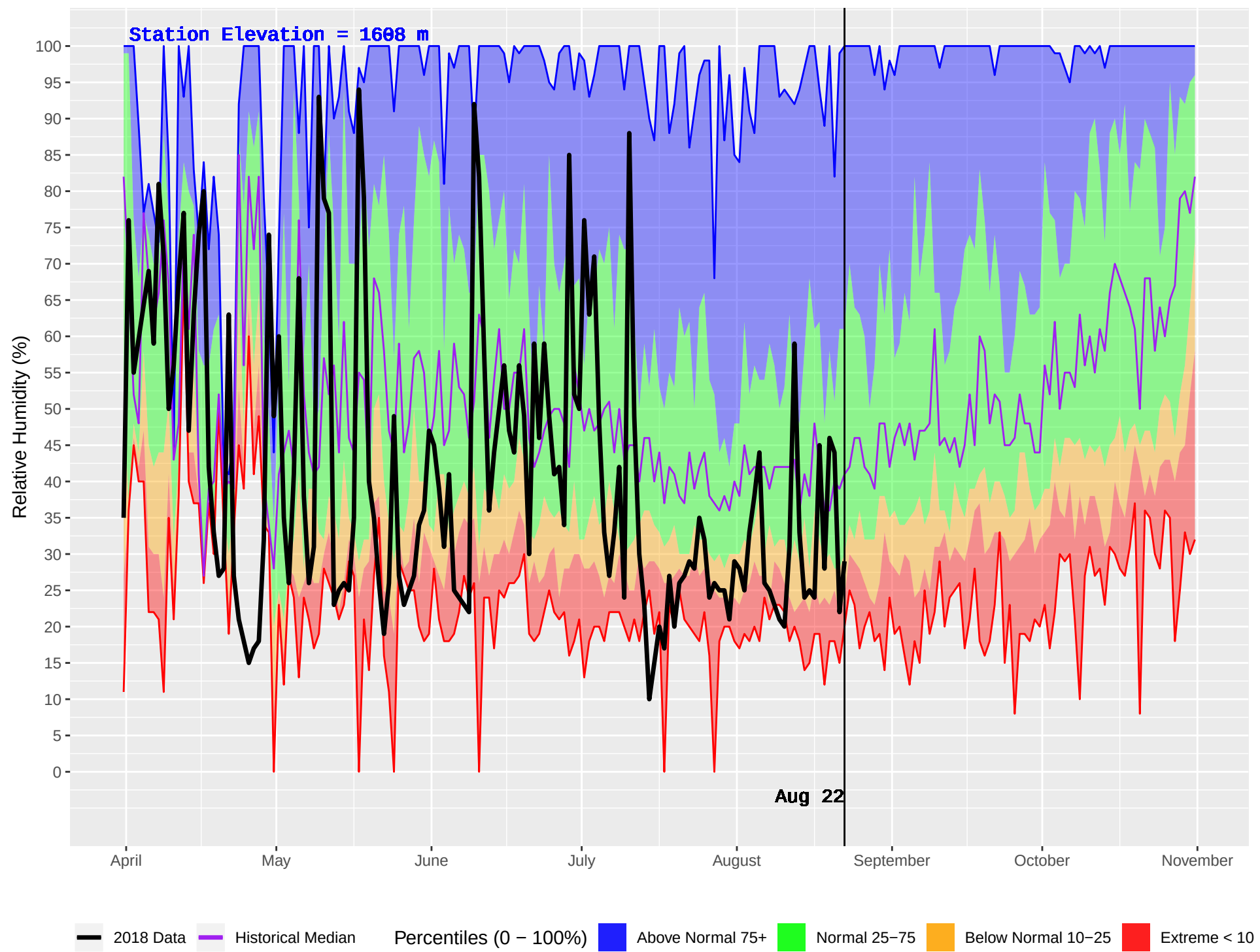
DEWAR CREEK (421) : Historical (1986–2016) and Current (2018) Daily Relative Humidity
