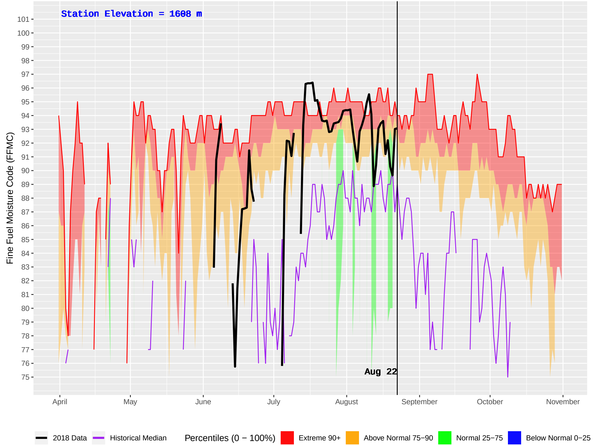
DEWAR CREEK (421) : Historical (1986–2016) and Current (2018) Daily Fine Fuel Moisture Code (FFMC)
