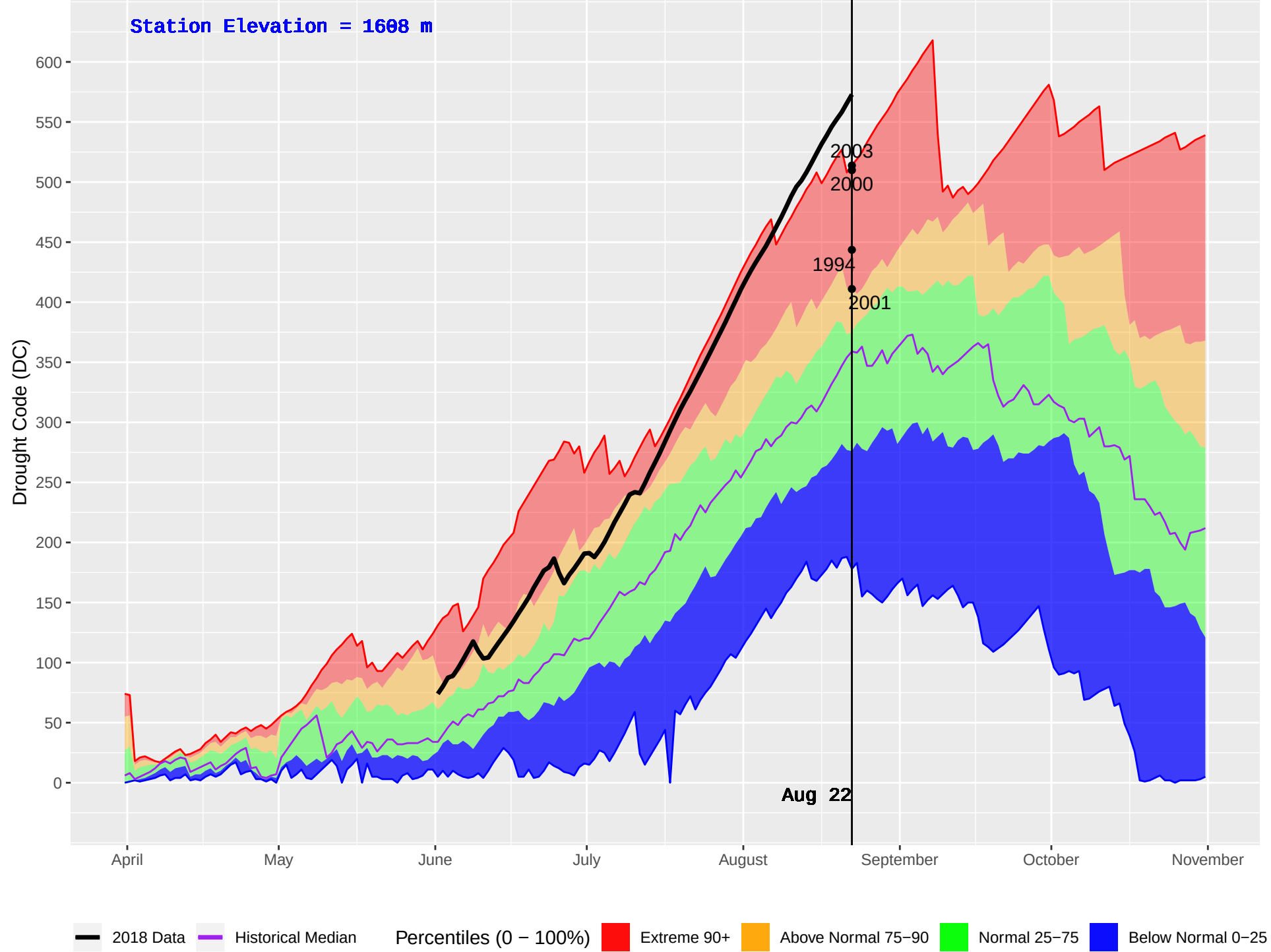
DEWAR CREEK (421) : Historical (1986–2016) and Current (2018) Daily Drought Code (DC)
